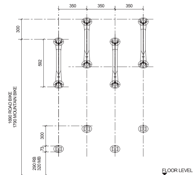
ELEVATION VIEW
